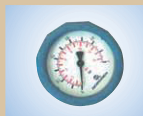
Manometer with protective casing (Ø63 mm – scale 0-1,0 bar), item no. .... 096041
